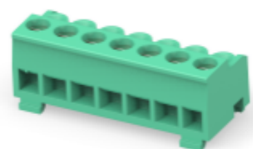
TE Part # 1546173-7 5MM PLUG, 90/180, 7 POS, GREEN, SN
