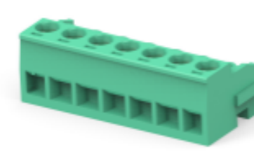
TE Part # 1986945-7 TERMI-BLOK PLUG 90&270DEG 5MM MODUL 7P
